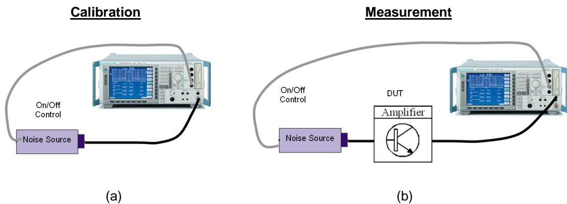
Figure 5: Connection diagram for (a) the calibration step, and (b) the measurement of the DUT's noise figure.
