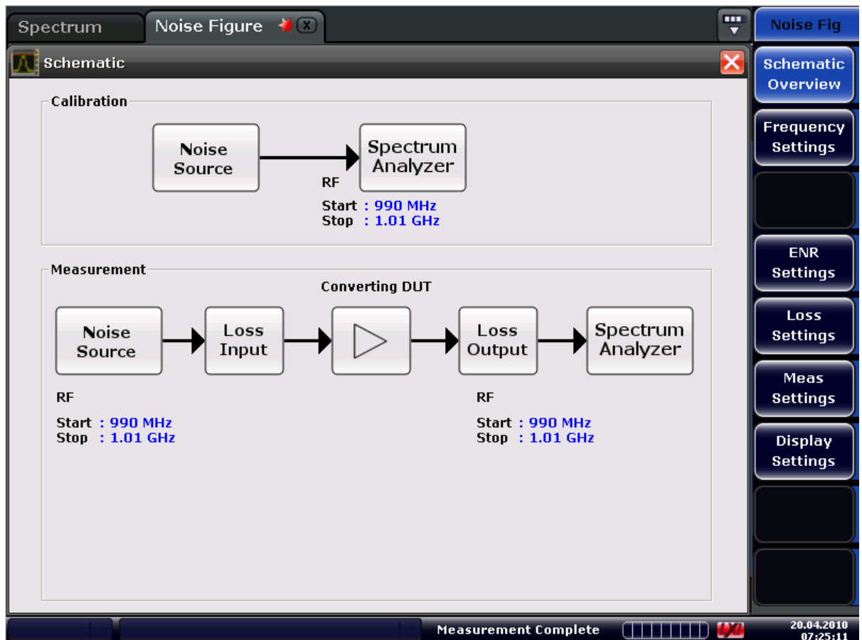
Figure 6: Configuration window for making noise figure measurements on a Rohde & Schwarz FSV spectrum analyzer
