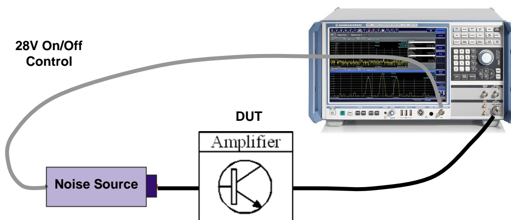
Figure 2: Common Setup to Measure Noise Figure.
