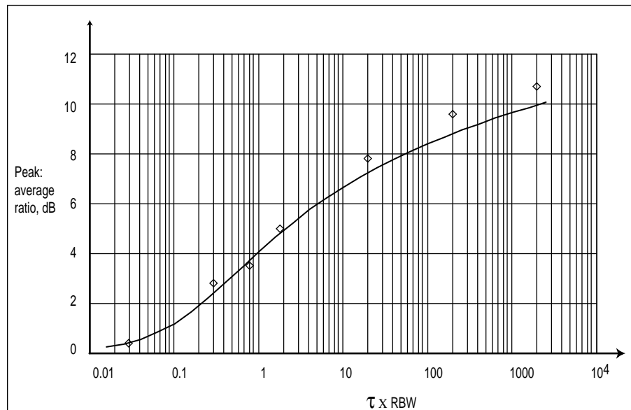
Figure E: The peak-detected response to noise increases with the observation time.
