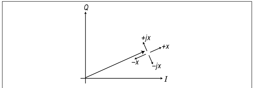
Figure G: Noise components can be projected into in-phase and quadrature parts with respect to a signal of unity amplitude and arbitrary phase.
