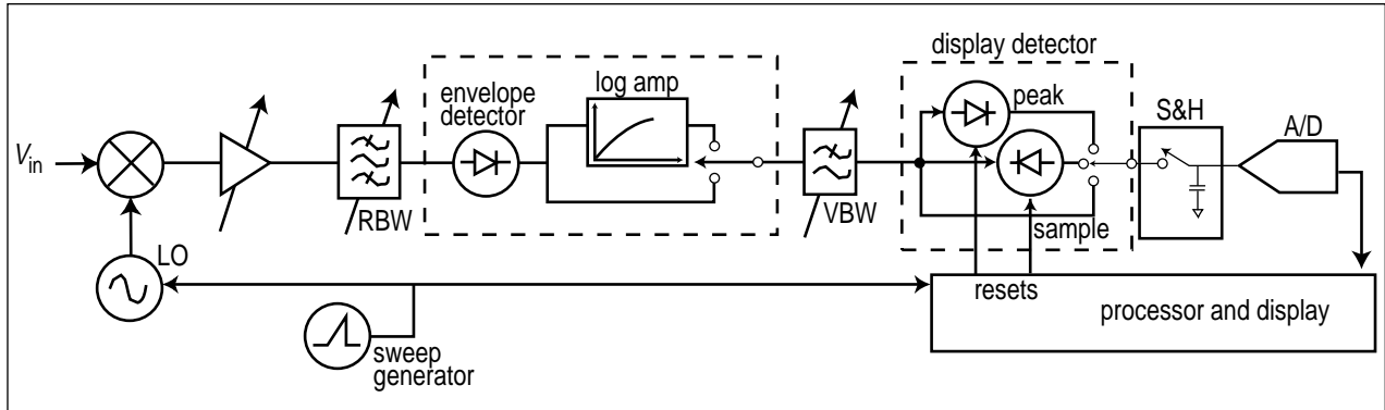
Figure A: Simplified spectrum analyzer block diagram
