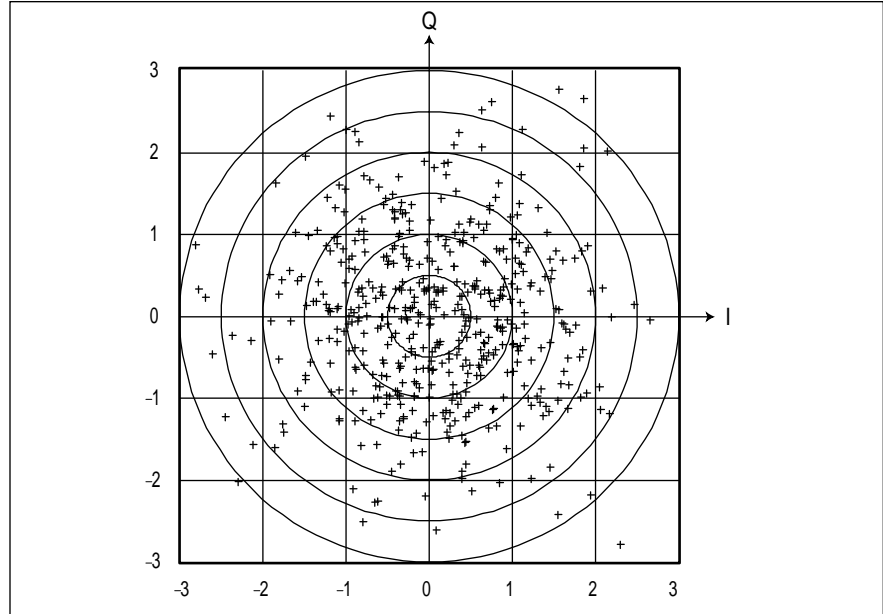
Figure 3: Samples of I/Q pairs shown with evenly spaced constant-amplitude envelope circles.
