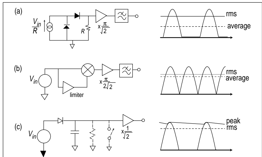
Figure B: Detectors: a) half-wave, b) full-wave implemented as a “product detector”, c) peak. Practical implementations usually have their gain terms implemented elsewhere, and implement buffering after the filters that remove the residual IF carrier and harmonics. The peak detector must be cleared; leakage through a resistor or a switch with appropriate timing are possible clearing mechanisms.
