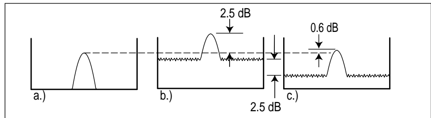
Figure 11: Log averaging improves the measurement of CW signals when their amplitude is near that of the noise. (a) shows a noise-free signal. (b) shows an averaged trace with power-scale averaging and noise power 1 dB below signal power; the noise-induced error is 2.5 dB. (c) shows the effect with log-scale averaging—the noise falls 2.5 dB and the noise-induced error falls to only 0.6 dB.
