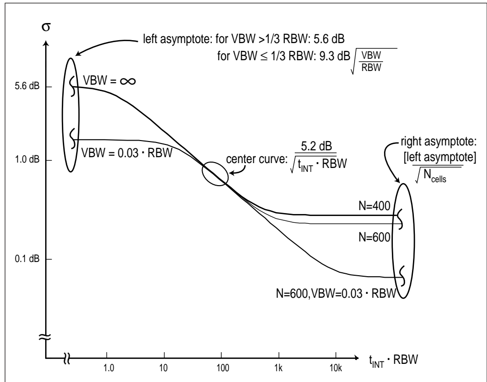
Figure 10: Noise measurement standard deviation for log-response spectrum analysis depends on the sweep-time/RBW product, the VBW/RBW ratio, and the number of display cells.
