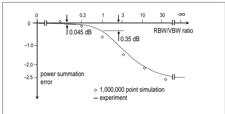
Figure 9: For \text{VBW} \geq 3\text{RBW} , the averaging effect of the VBW filter does not significantly affect power-detection accuracy.
