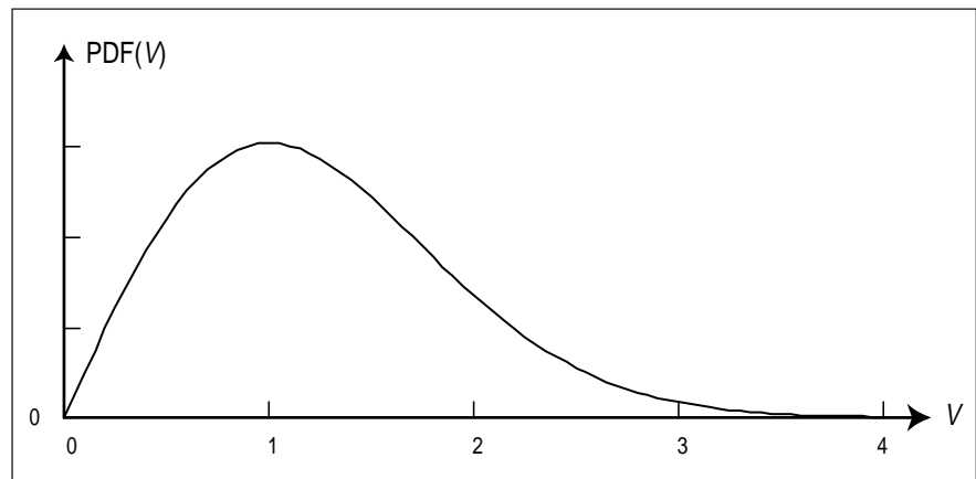
Figure 4: The PDF of the voltage of the envelope of a noise signal is a Rayleigh distribution. The PDF is zero at zero volts, even though the PDFs of the individual I and Q components are maximum at zero volts. It is maximum for v = \text{sigma} .
