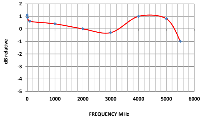
BBGen-pulse typical output flatness
